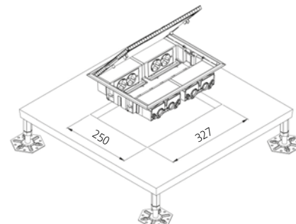
4 modules doubles KF400/1
