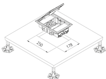
2 modules doubles KF200/1
