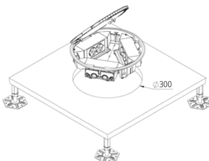
3 modules doubles KF300C/1
